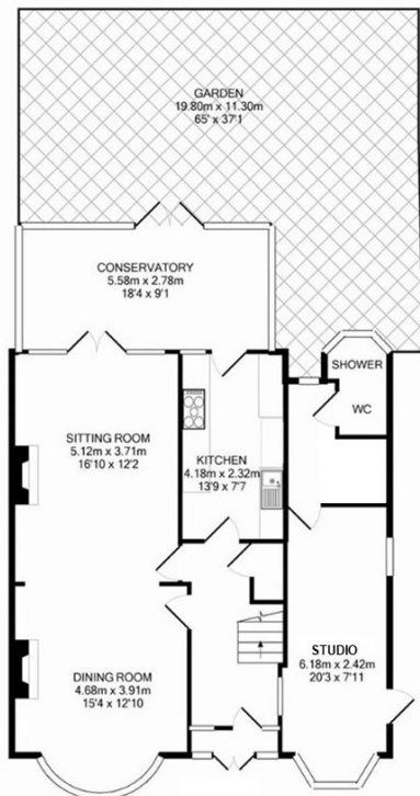
Ground Floor Approx. Floor Area 92.2 sq m / 992 sq ft
